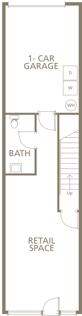
ENTRY FIRST FLOOR
